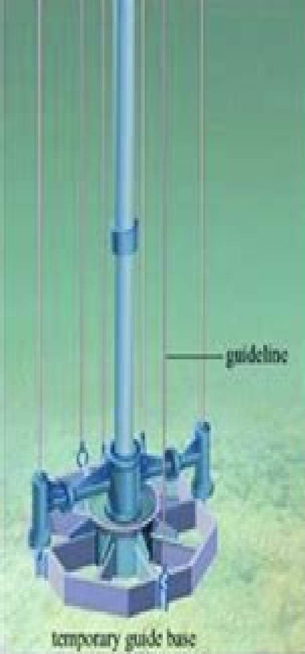
Temporary guide base
