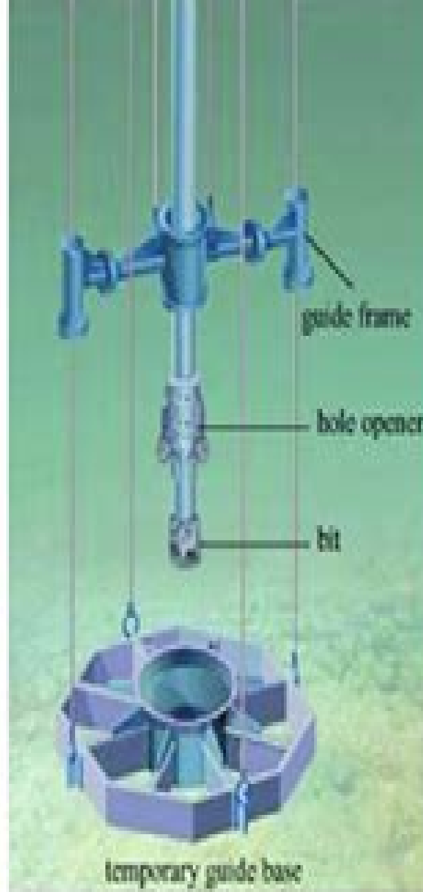
Guide frame for the drill string
