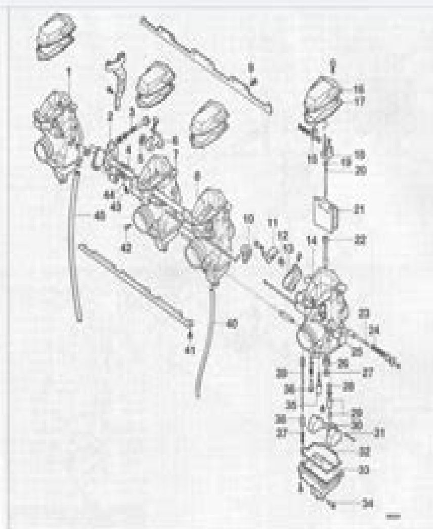
61 W800 carburetor - exploded view
