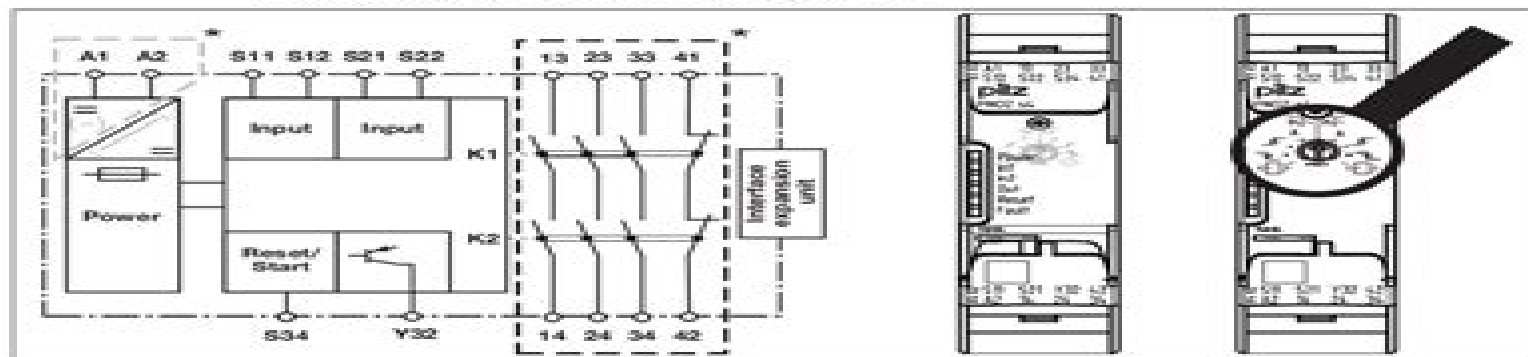
Fig.: Rotary cam arrangement monitoring Front view with cover, right: Front view without cover
