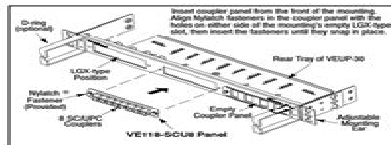
Figure 2. Installing VE118-SCU8 Panel in a VEUP-30
