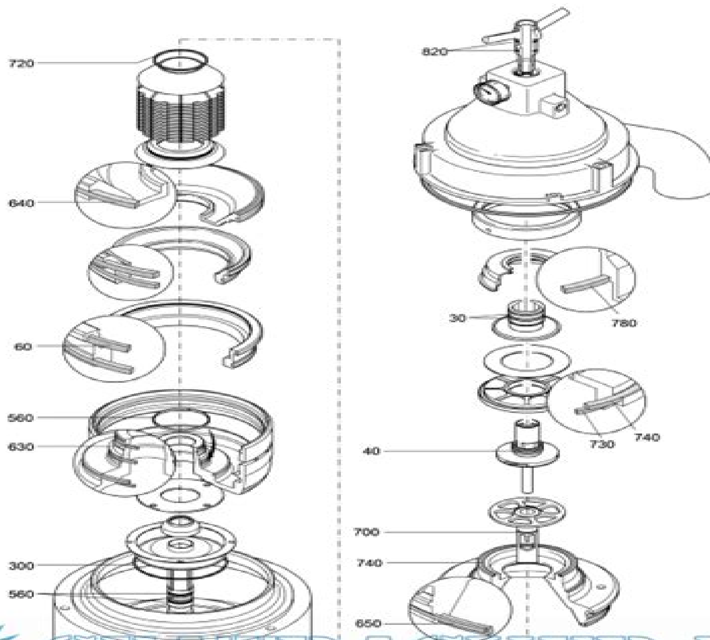
Fig. 1.11 Set of spare parts „bowtmodel“ (operation: 1 year or 8,000 hours)
