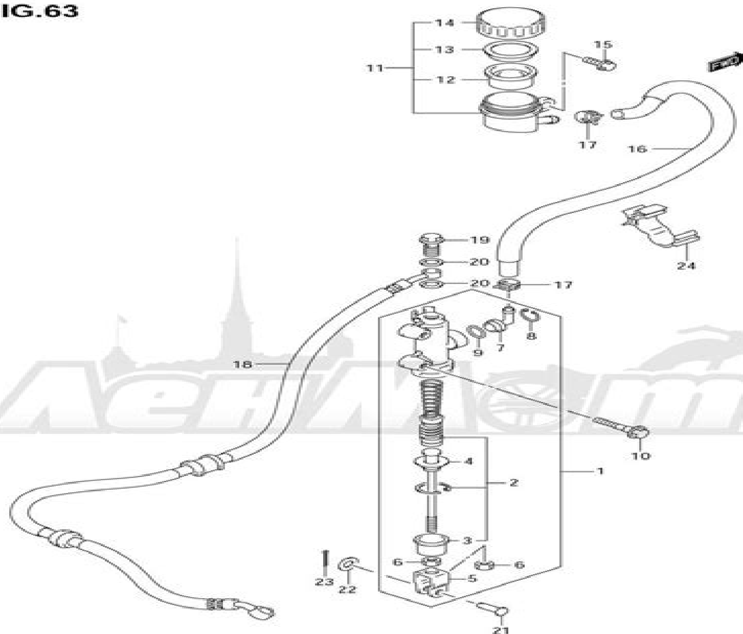
LT-F500FK4 P28 P33_063 REAR MASTER CYLINDER
