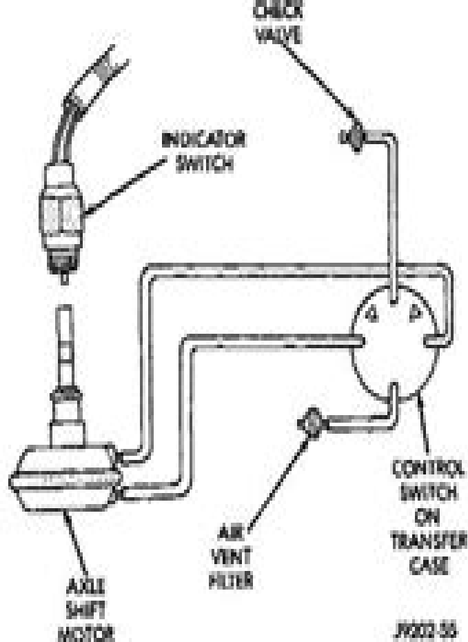
Fig. 5 Vacuum Control System
