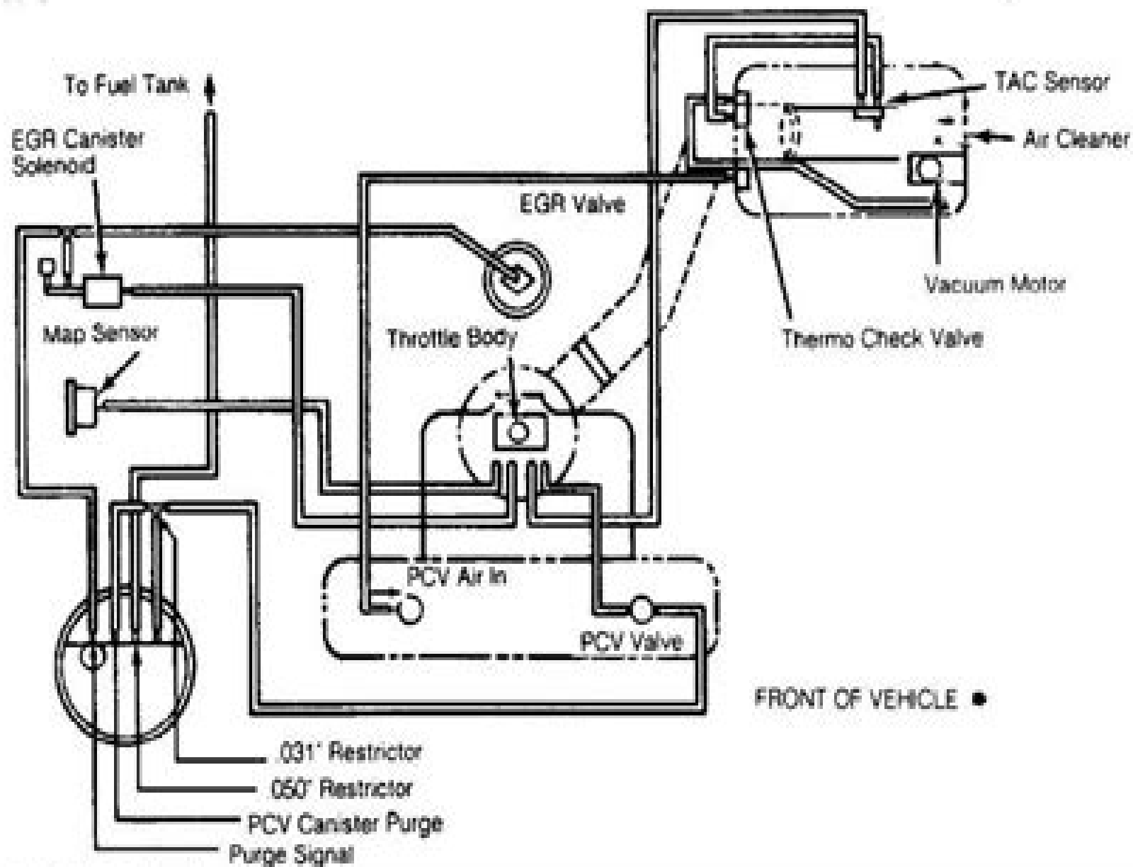
Fig. 1: 2.5L 4-Cylinder
