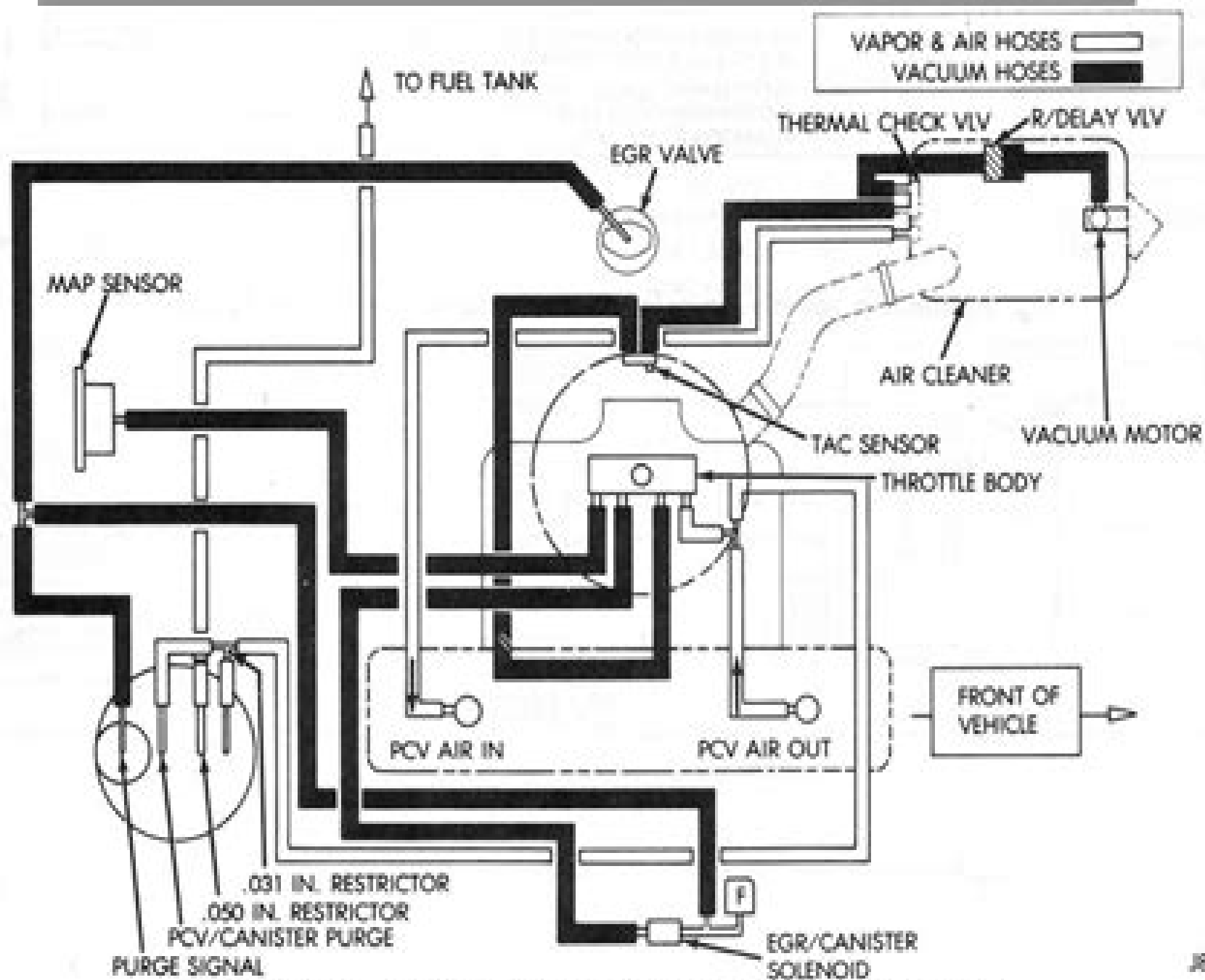
Fig. 8 Emissions Schematic—YJ Vehicles with 2.5L Engine
