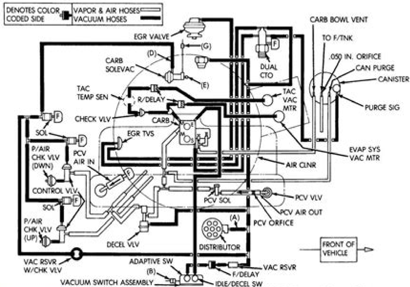
Pressauto.NET Fig. 11 Emissions Schematic—YJ Vehicles with 4.2L Engine and Manual Trans.
