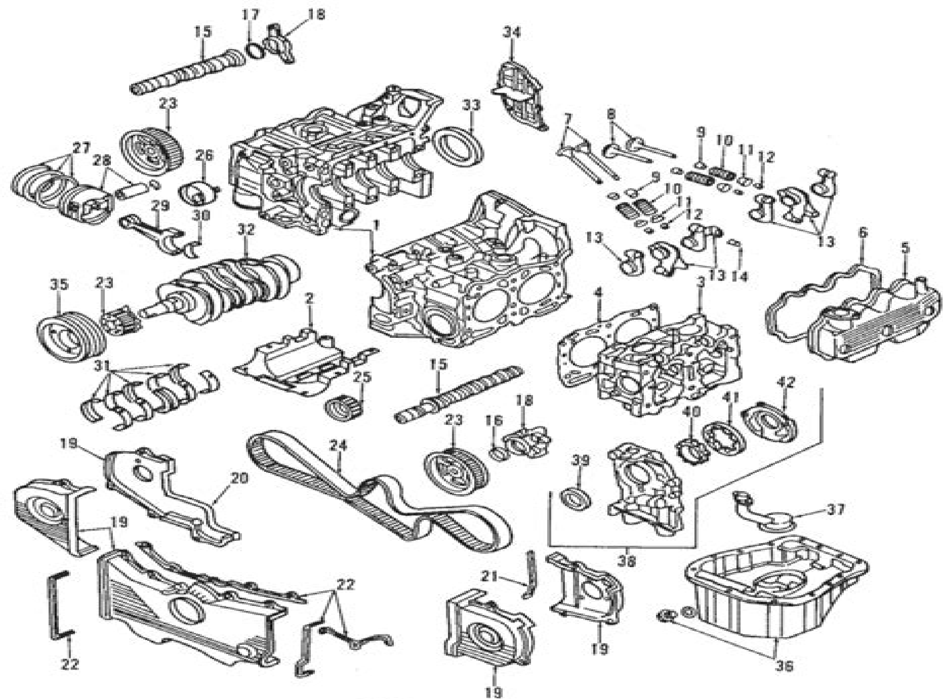
ENGINE-2.2 LITER
