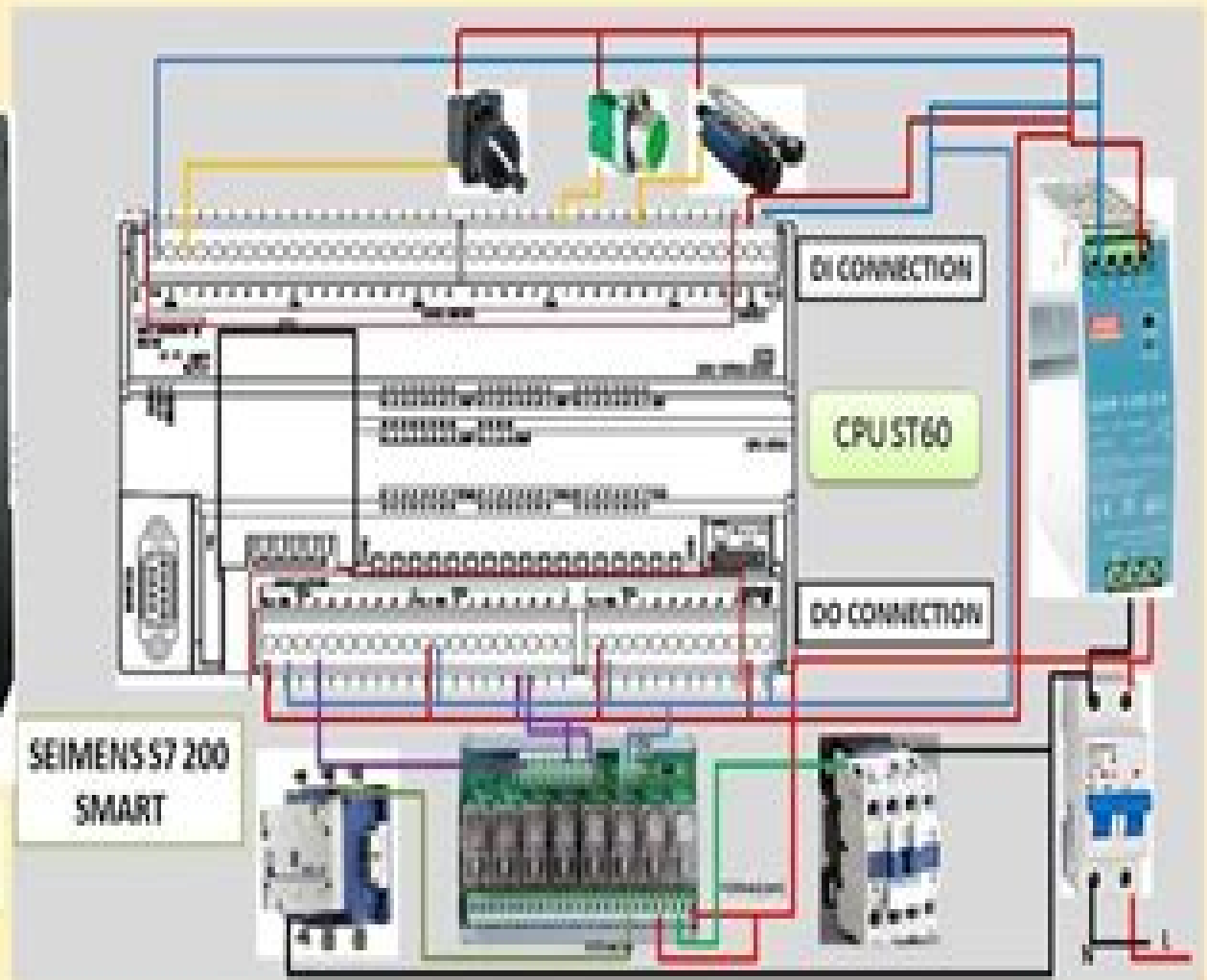
S7 200 - CPU ST60
