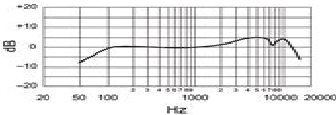
Frequency Response
