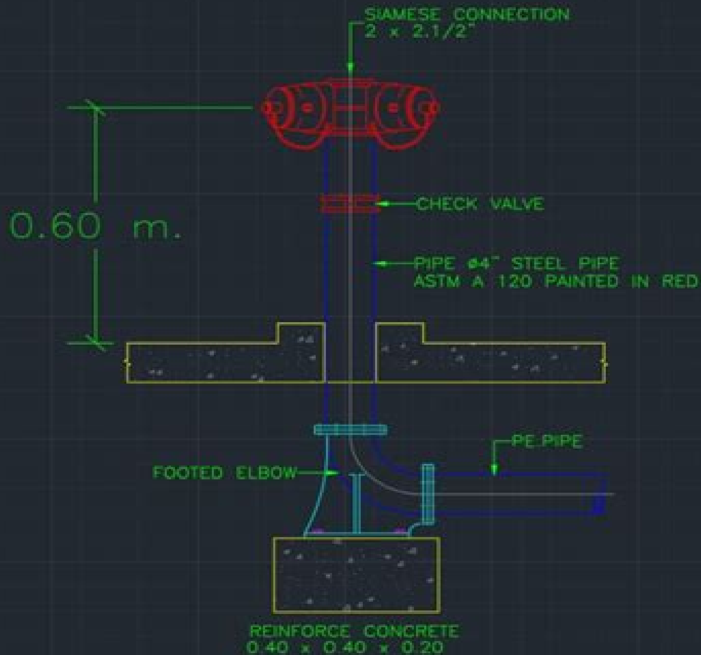
SIAMESE CONNECTION
