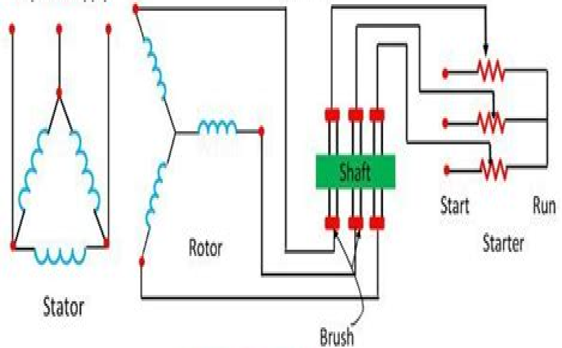
Slip Ring Induction Motor
