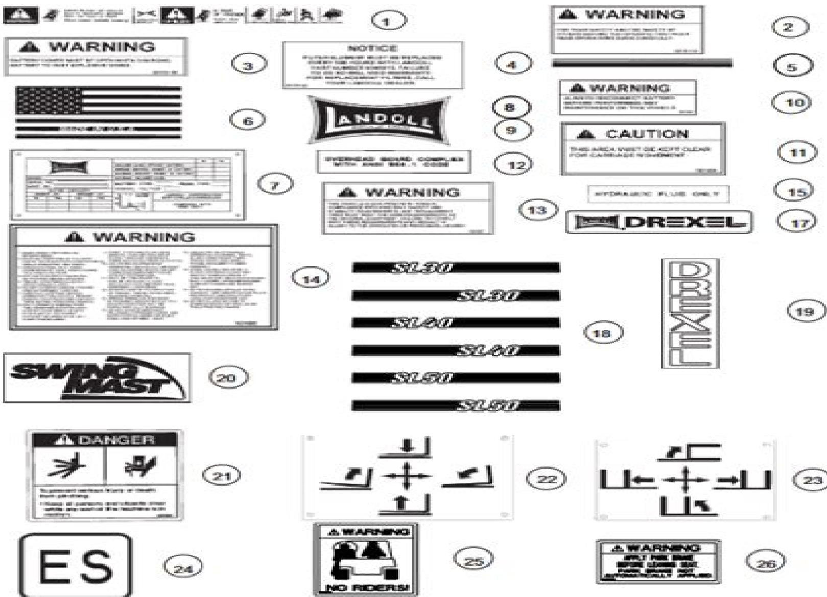
Figure 5-3 SL Series Decals
