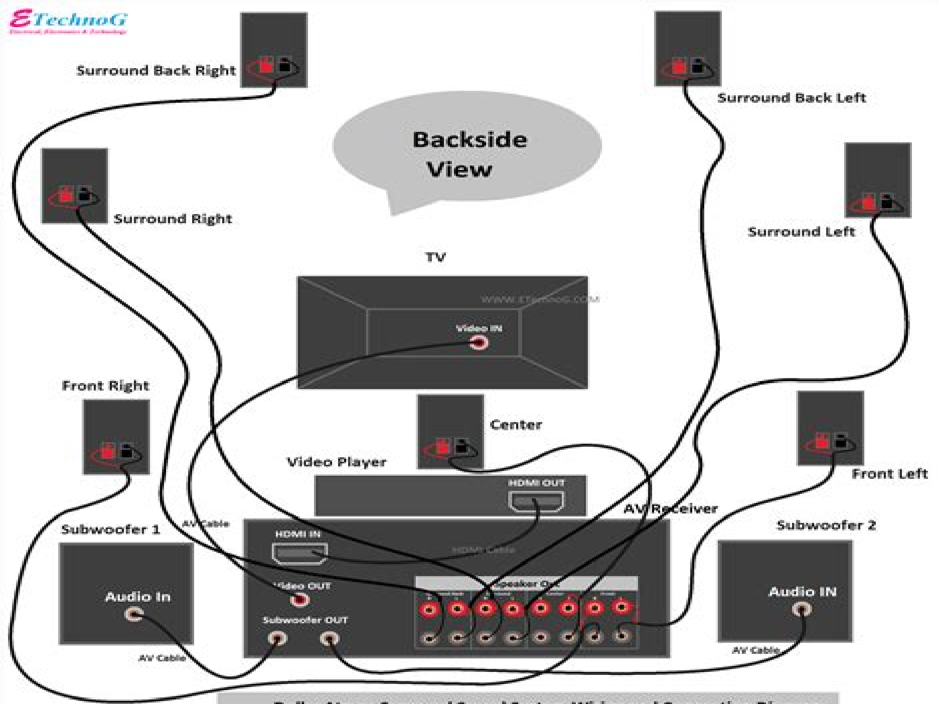
Dolby Atmos Surround Sound System Wiring and Connection Diagram
