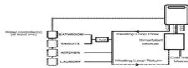
(Fig. 5) - Not a 50°C Appliance. Note: TLD = Temperature Limiting Device
