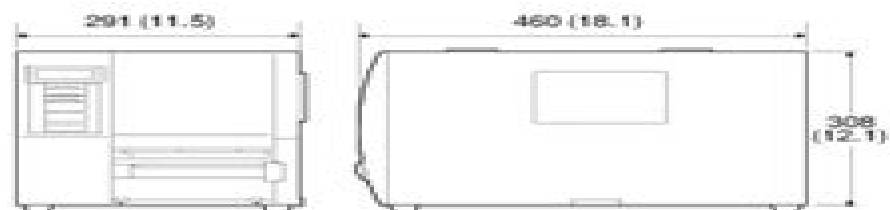
Dimensions in mm (inches)
