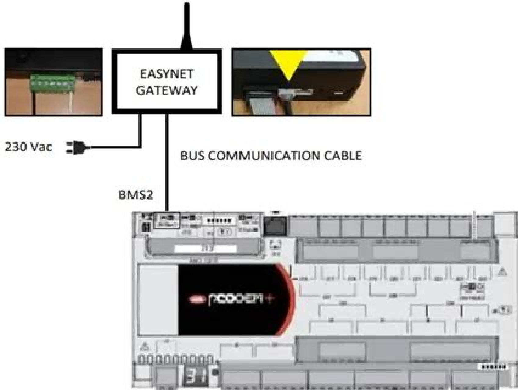
Figure 3.1. Installation of the EASYNET GATEWAY to the ECOFOREST device.
