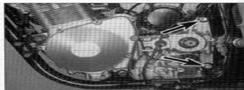
5.20d ... then withdraw the rear mounting bolts (arrows) ...
