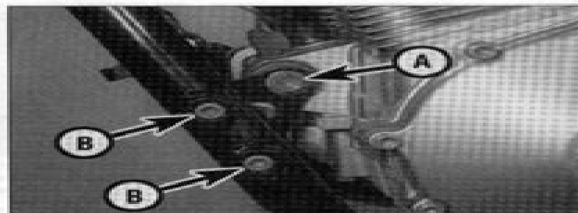
5.20b ... then remove the engine front bolt (A) and the bracket bolts (B), and remove the bracket
