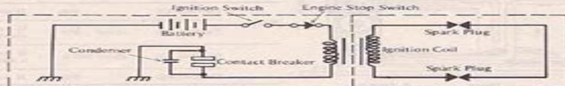
Ignition circuit wiring
