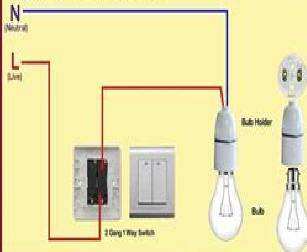
[02] 2 Gang 1 Way Switch Connection
