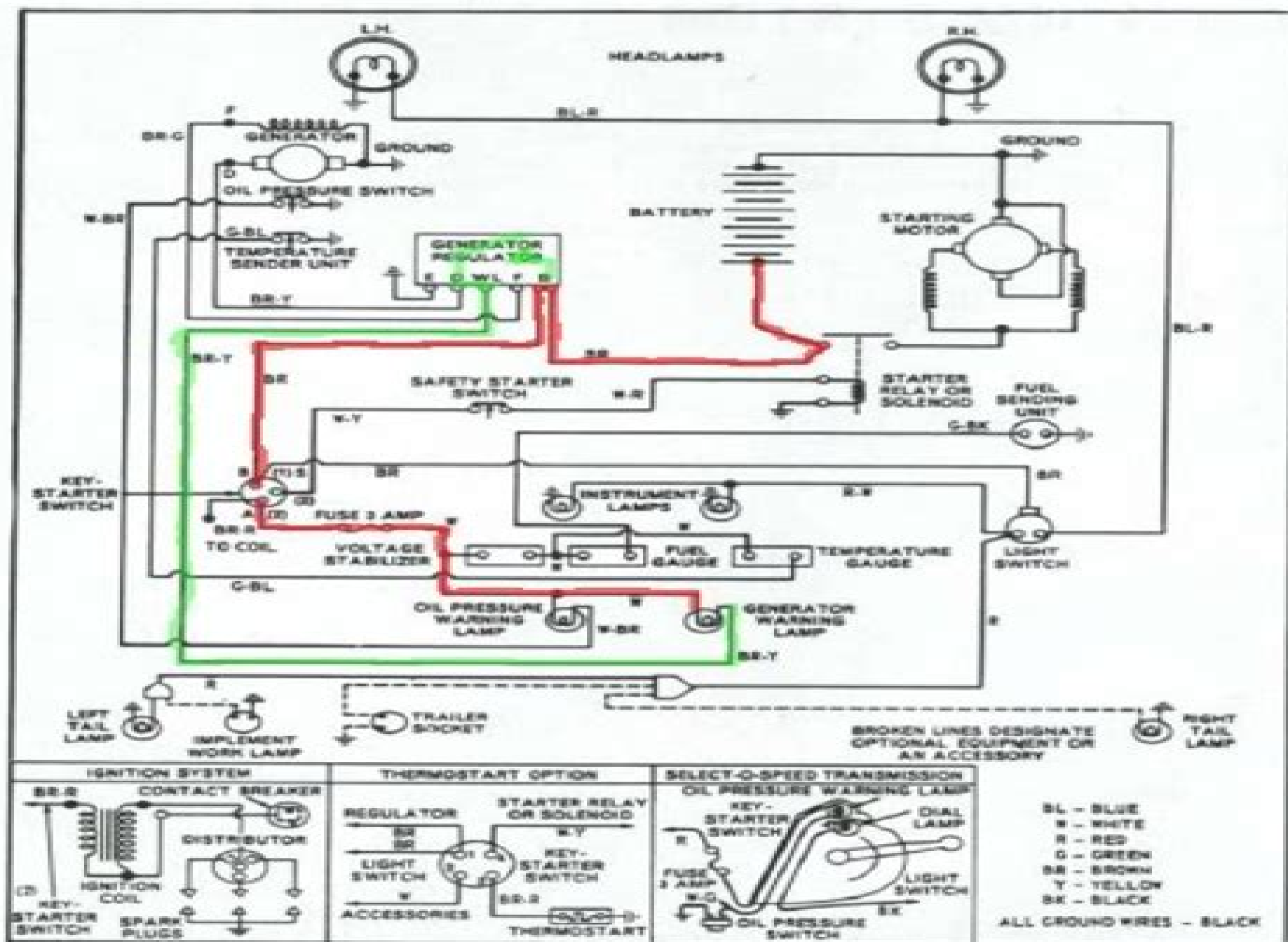
Fig. 160—Wiring diagram for all models with "C" prefix to tractor serial number. Refer to page 2 of this manual for serial number location. For tractors with "A" or "B" prefix to tractor serial number,
