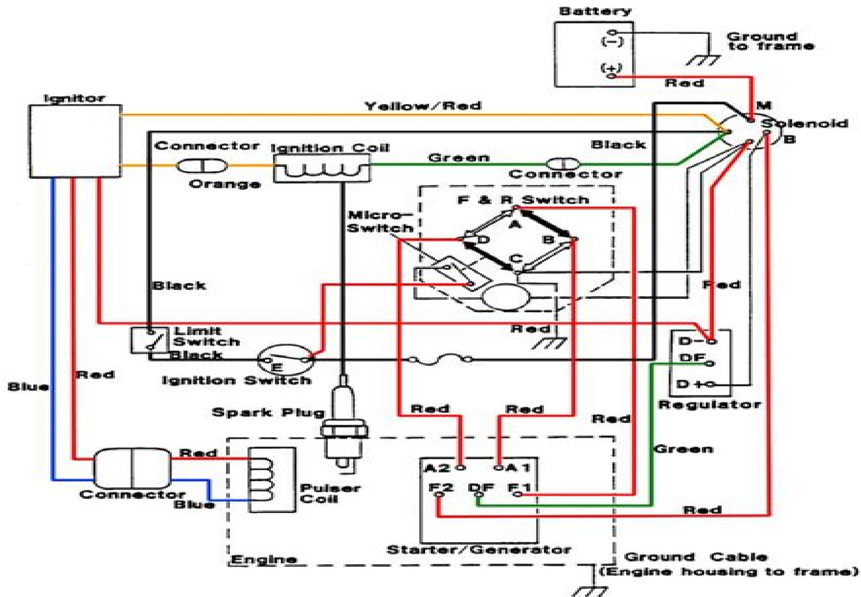
FIG. L-1 ELECTRICAL SYSTEM WIRING DIAGRAM
