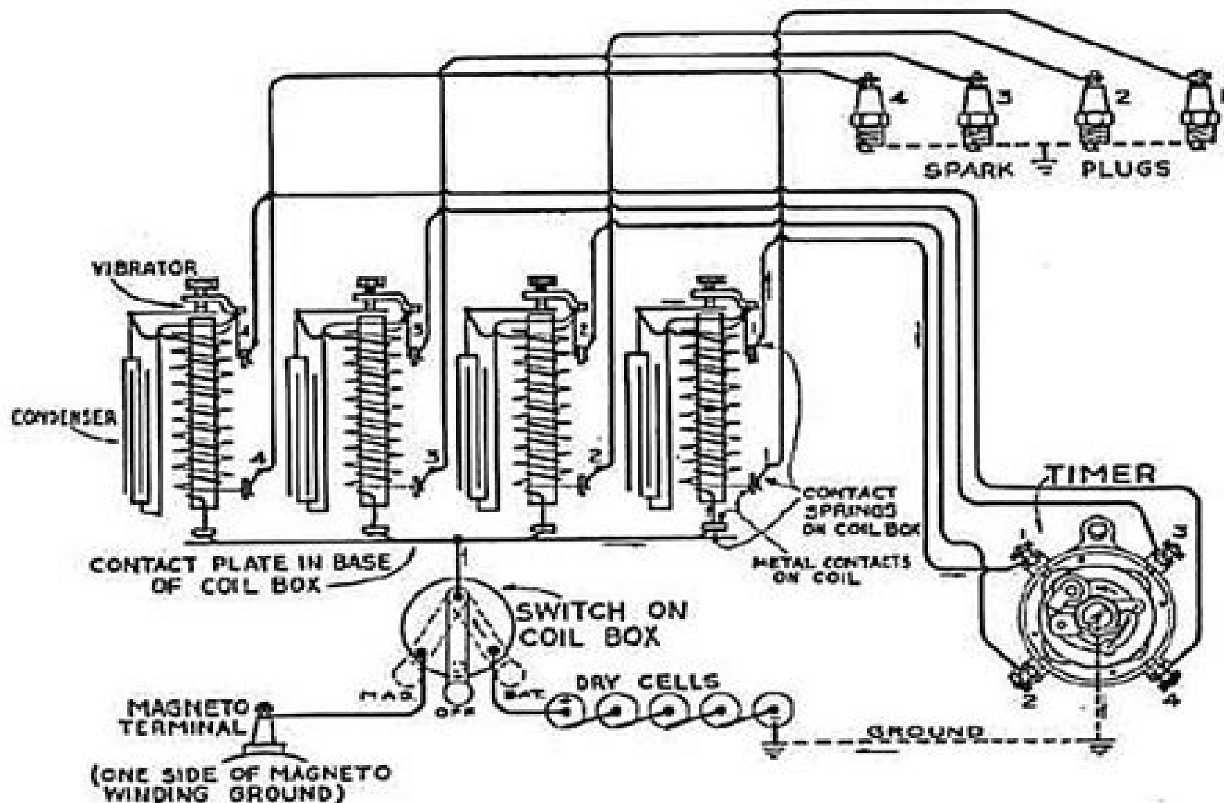
Figure 5—Simplified Diagram of Integrated Model T Ignition Components
