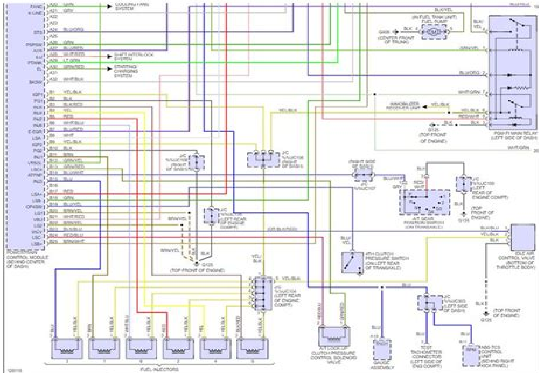
Fig 1: 3.2L Engine Performance Circuit (1 of 4)
