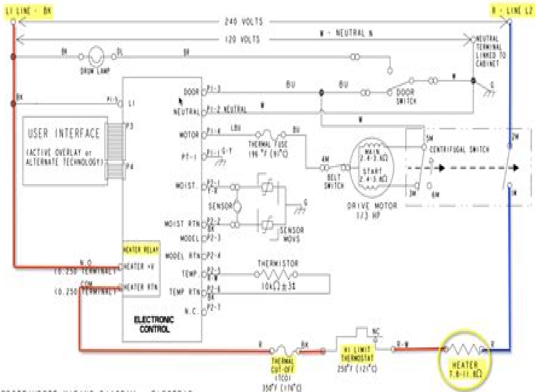
EDOTT/VDOTT WIRING DIAGRAM - ELECTRIC
