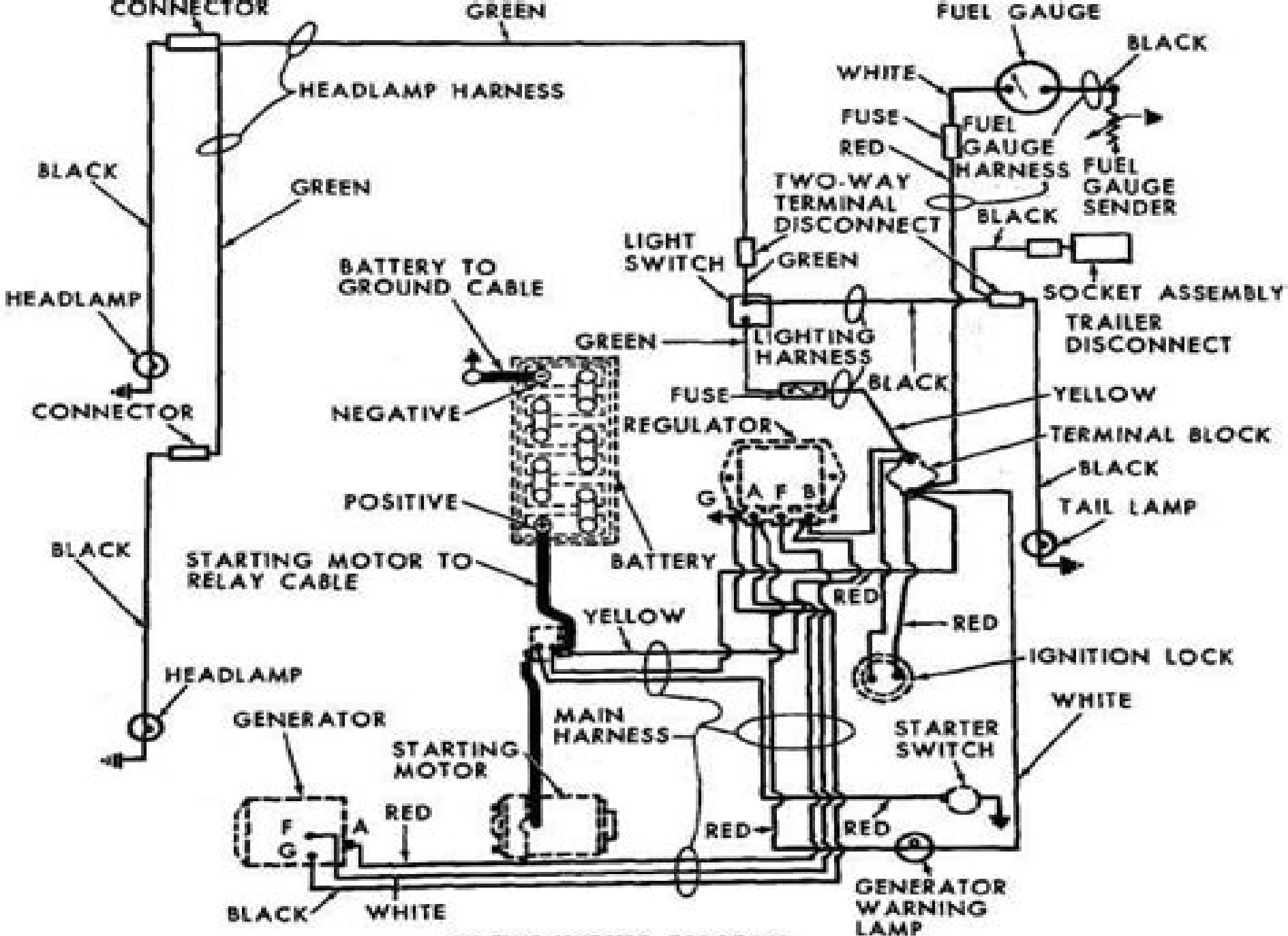
CIRCUIT WIRING DIAGRAM 12-VOLT SYSTEM
