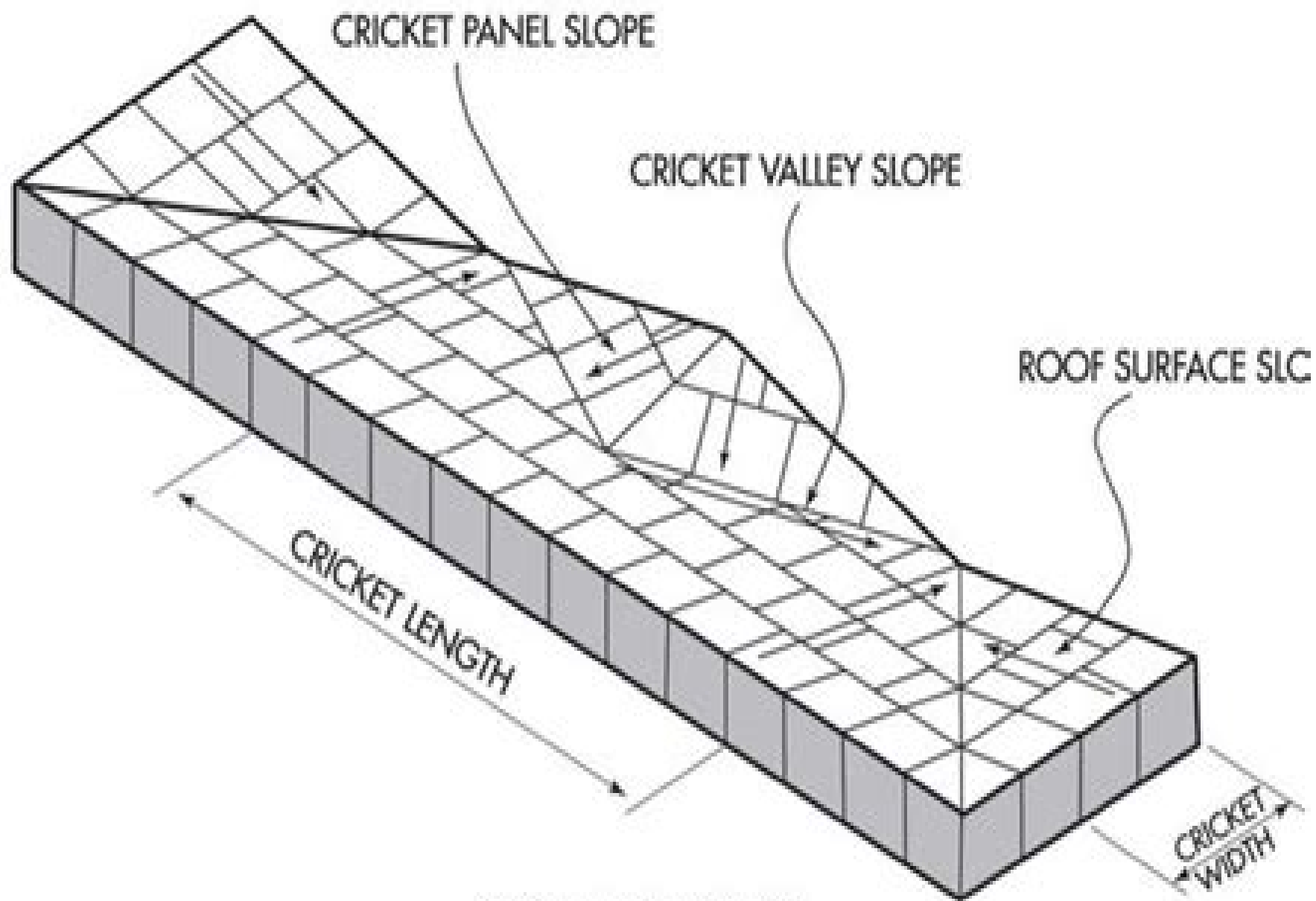
ISOMETRIC VIEW
