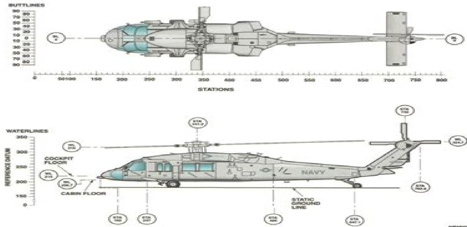
Figure 3-10. Fuselage Stations
