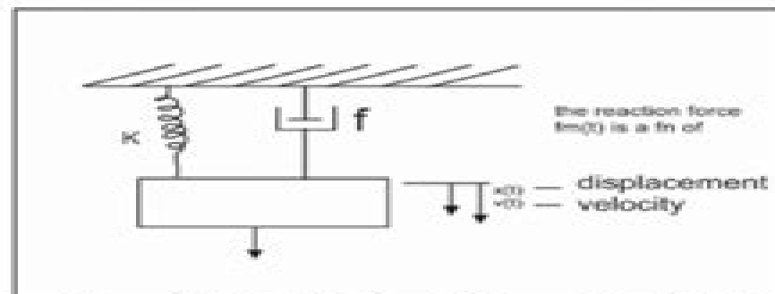
Figure 2.1: Basic Mechanical Translational System
